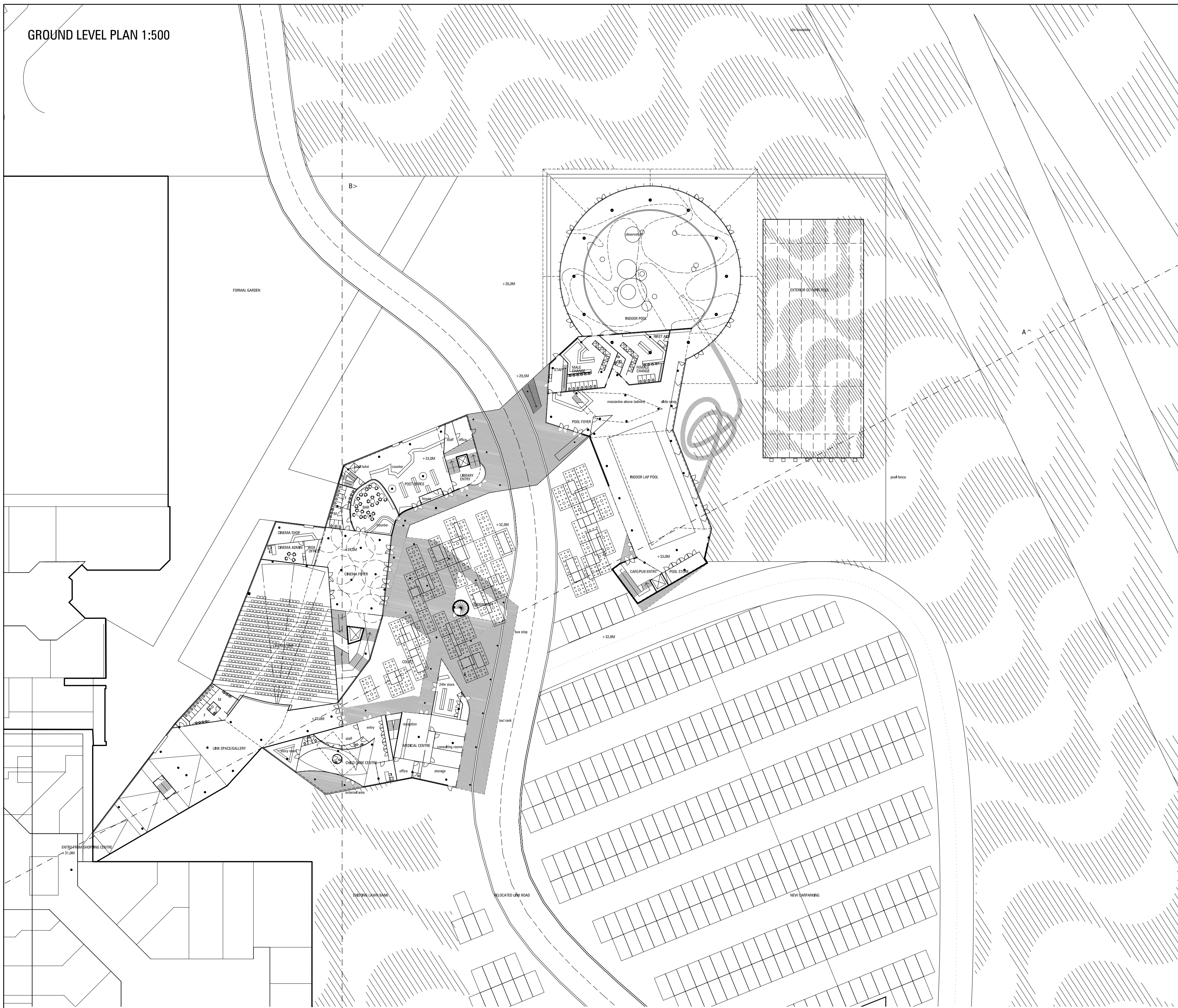
FIRST LEVEL PLAN 1:500
